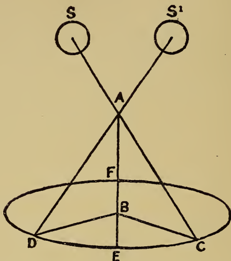
FIG. 12. To Find the Meridian by Sun.
